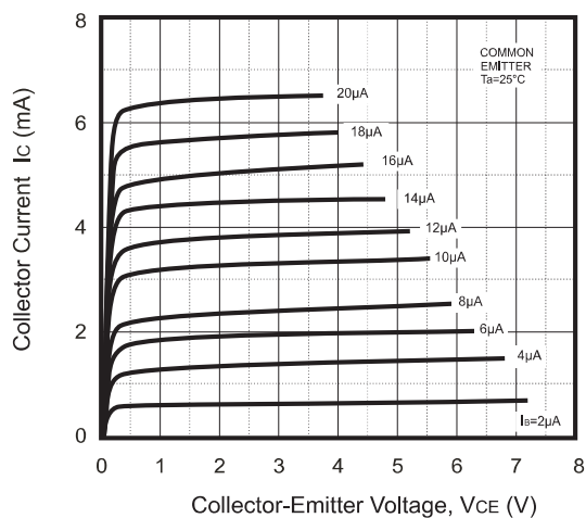
Fig.1 - Static Characteristic
